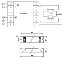
Specifications Philips HF-R 236 TL-D EII 220-240V for 2x36W
